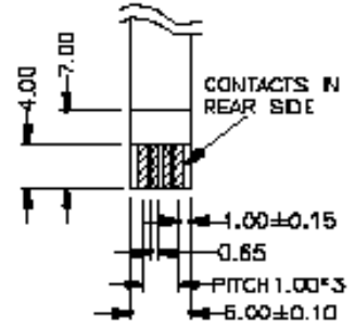
DETAIL A SCALE 2.0
